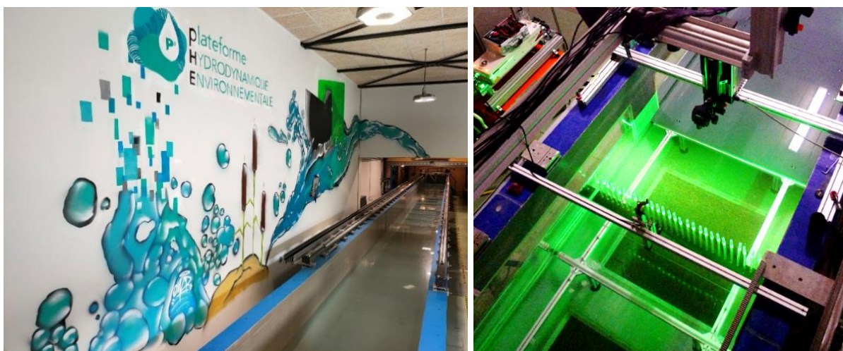
The hydrodynamic flume of the Environmental Hydrodynamics Platform (pHE) at the Institut Pprime (CNRS–University of Poitiers). PIV measurements of flow in fluid–structure interaction with a calibrated array of flexible stem models.
